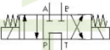
... now showing: P-T in neutral
