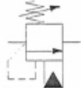
Overcentre valve (counter-balance valve)
