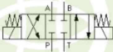
4/3 direct operated directional control valve: solenoid operated, spring centered, all ports closed in neutral...
