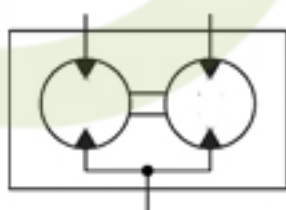
Rotary flow divider
